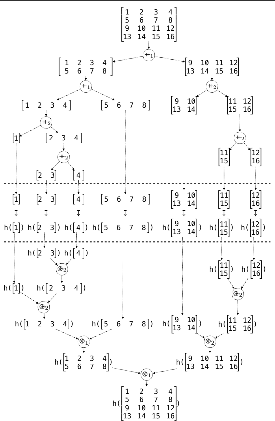
Fig. 10. MDH property recursively applied to a two-dimensional example computation
